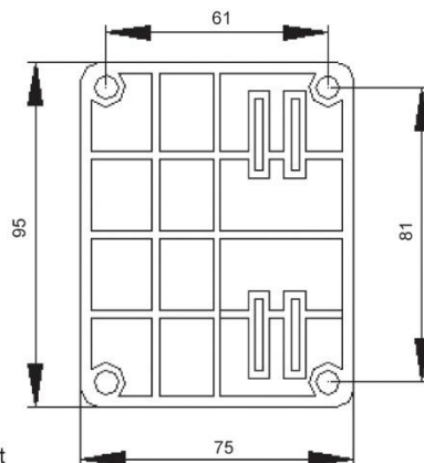
Mount bracket
